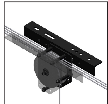
Head and Loft Block with ball bearings.
