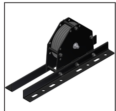
Head and Loft Block with tapered bearings.
