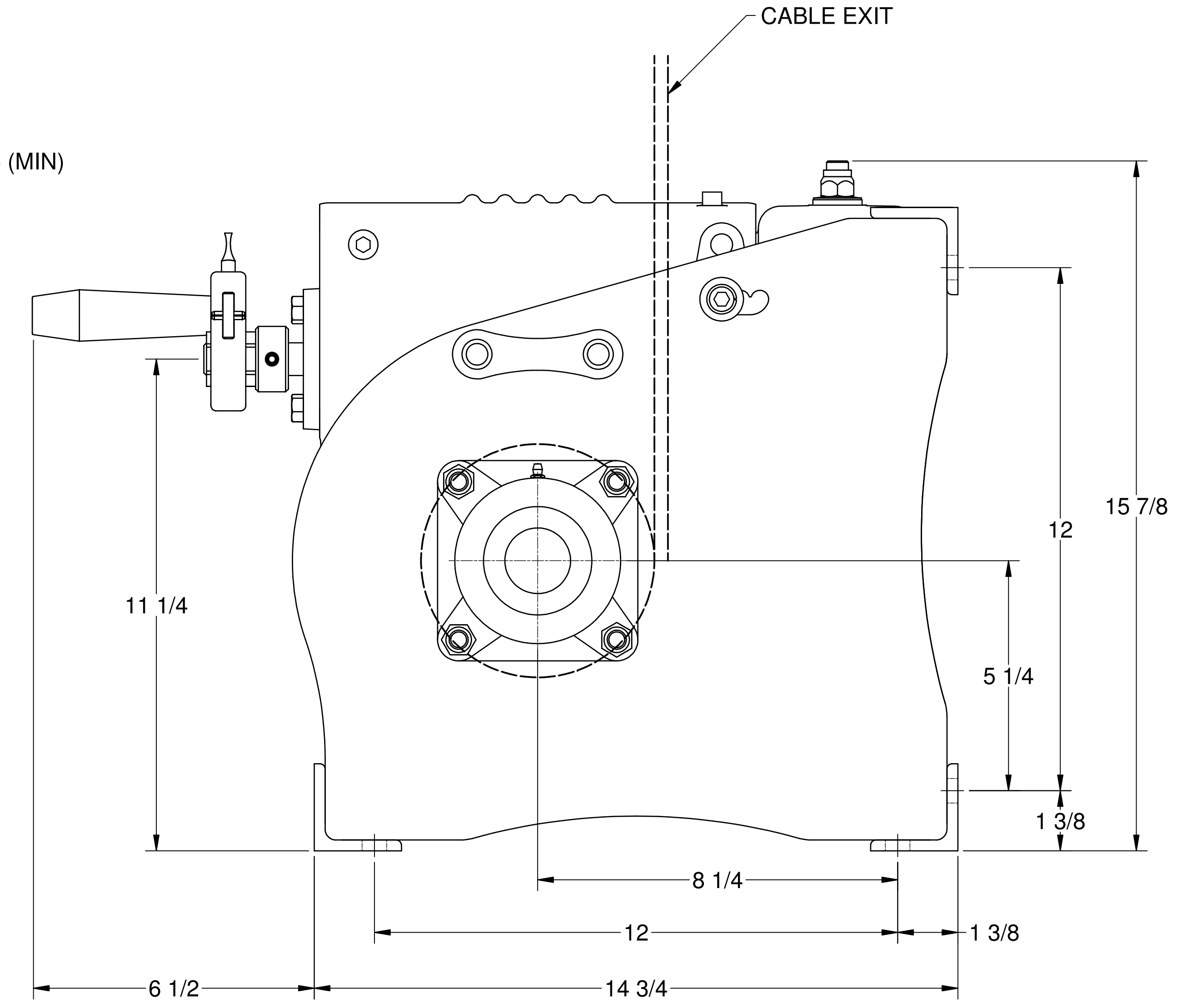
SIDE VIEW
