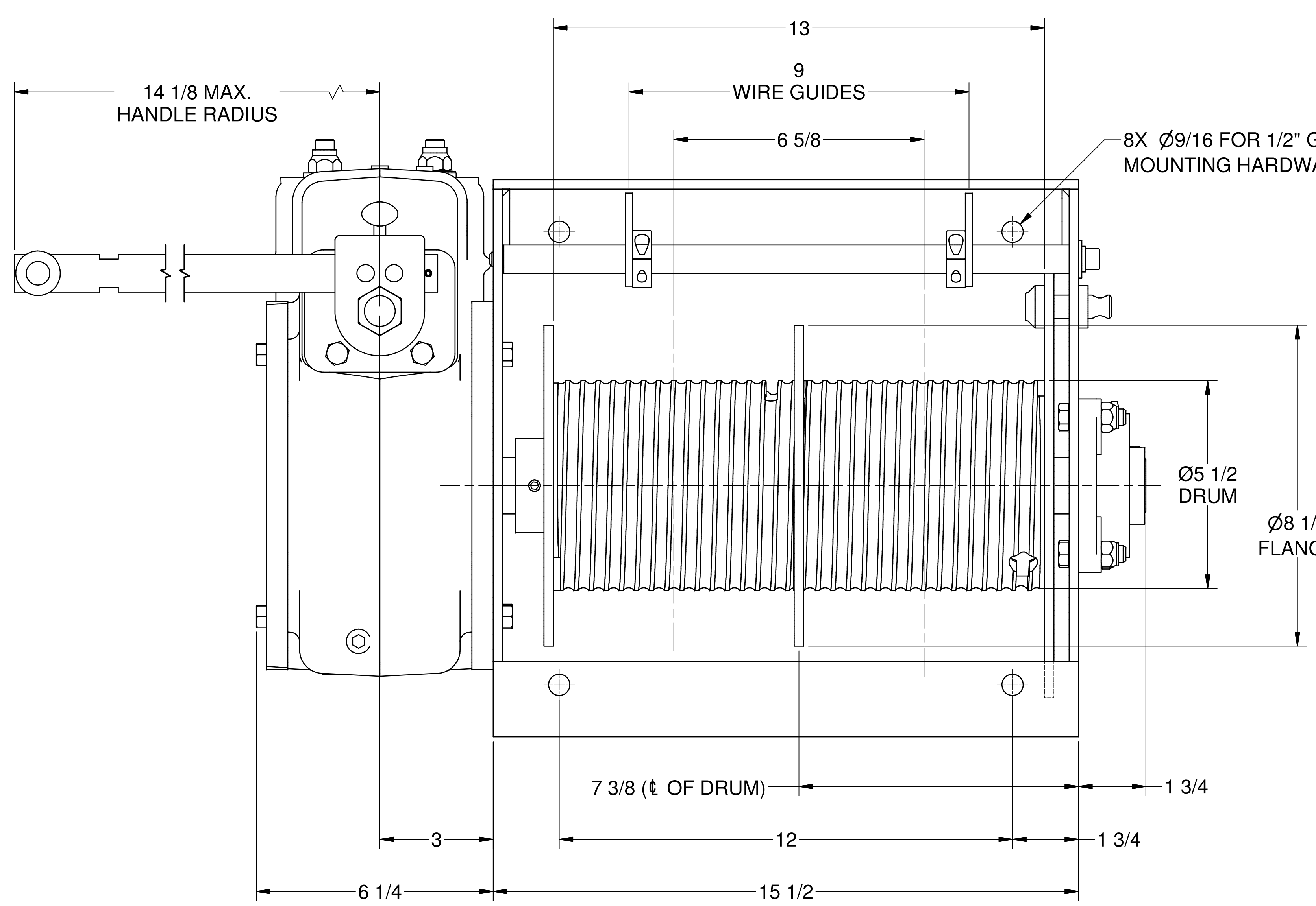
FRONT VIEW
